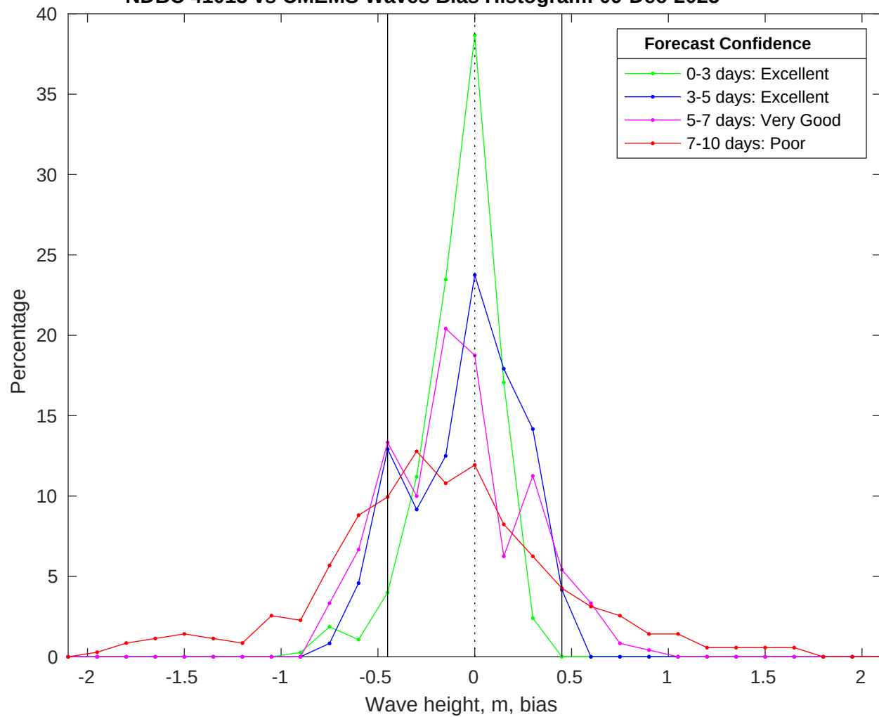
NDBC 41013 vs CMEMS Waves Bias Histogram: 09-Dec-2025
