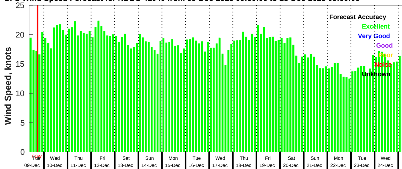
GFS Wind Speed Forecast for NDBC 41040 from 09-Dec-2025 09:00:00 to 25-Dec-2025 09:00:00
