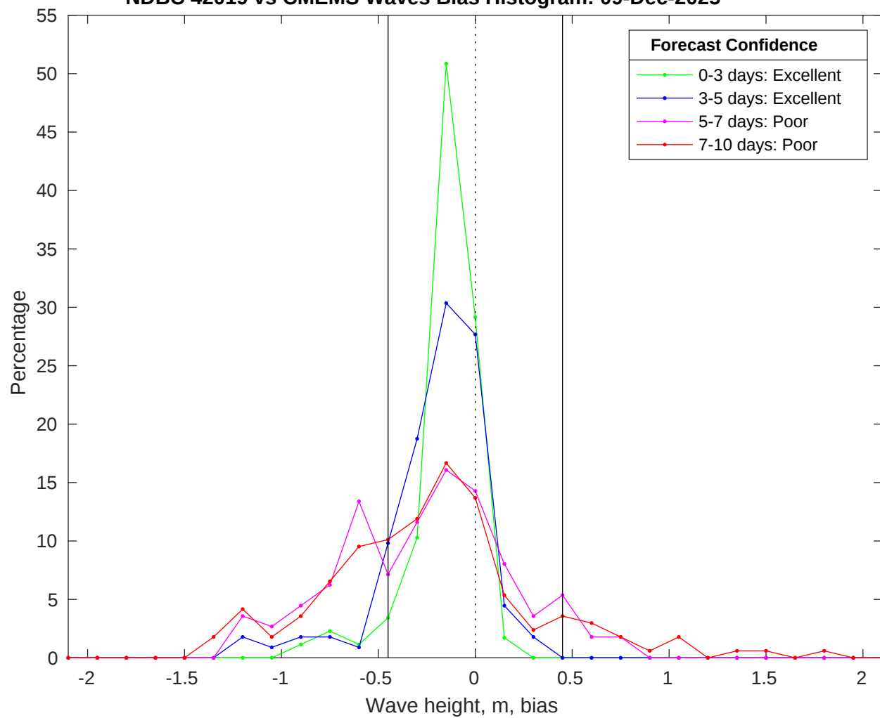
NDBC 42019 vs CMEMS Waves Bias Histogram: 09-Dec-2025
