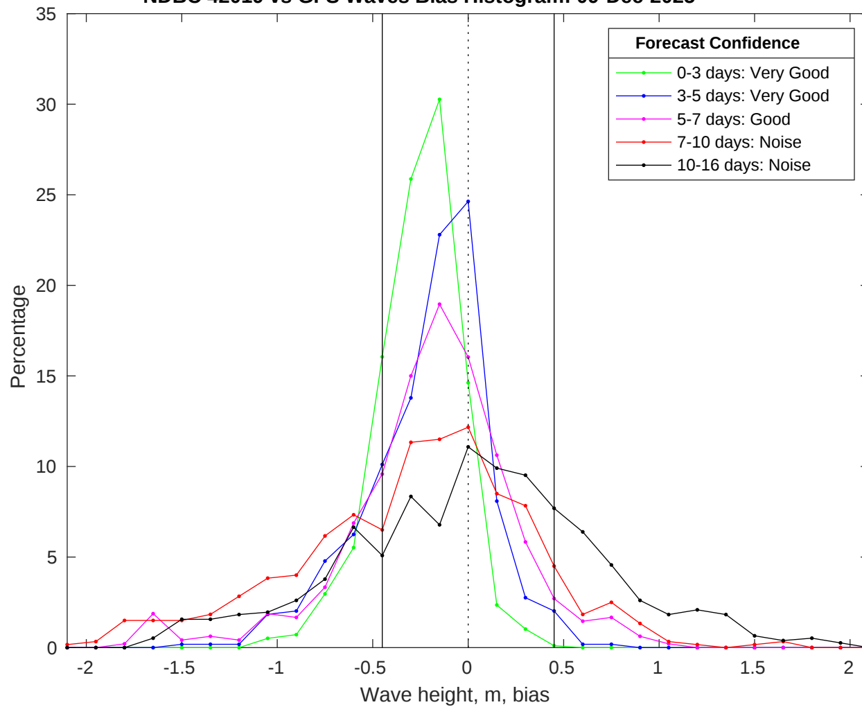
NDBC 42019 vs GFS Waves Bias Histogram: 09-Dec-2025
