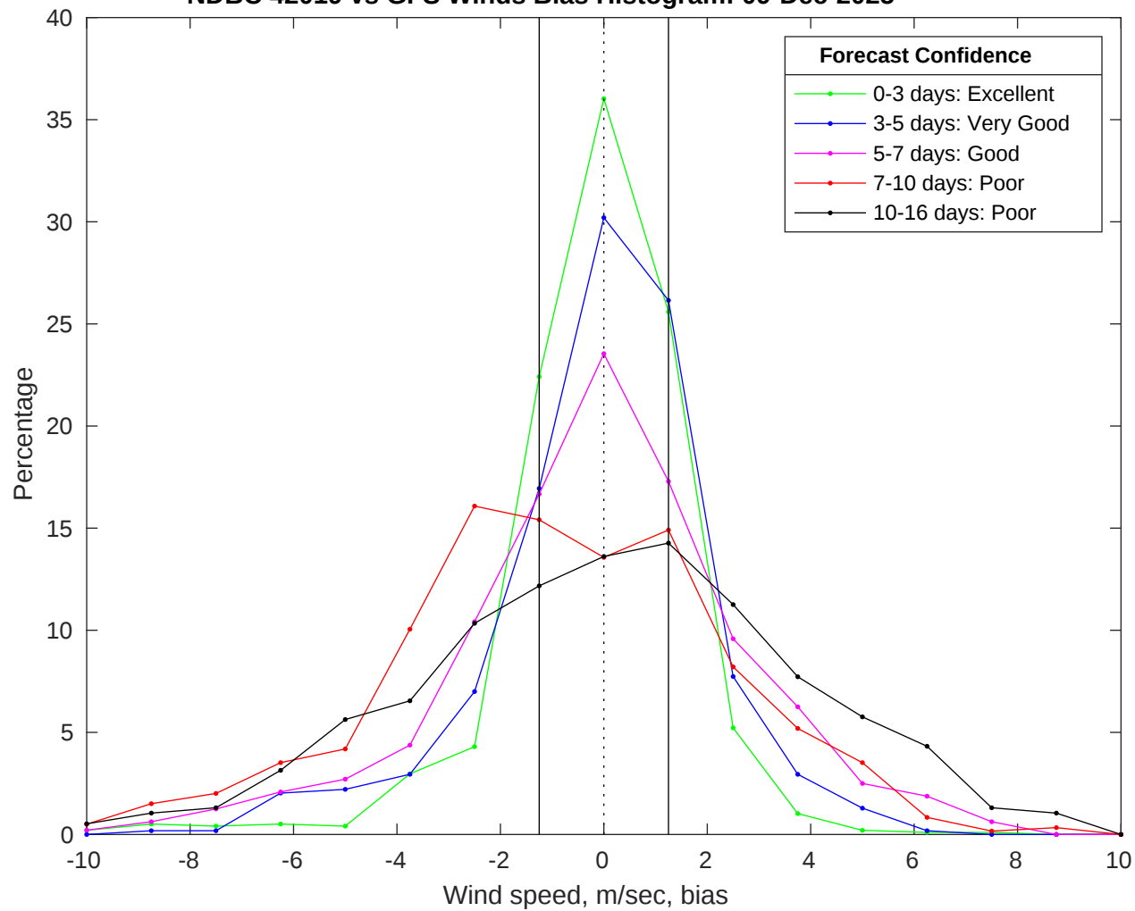
NDBC 42019 vs GFS Winds Bias Histogram: 09-Dec-2025
