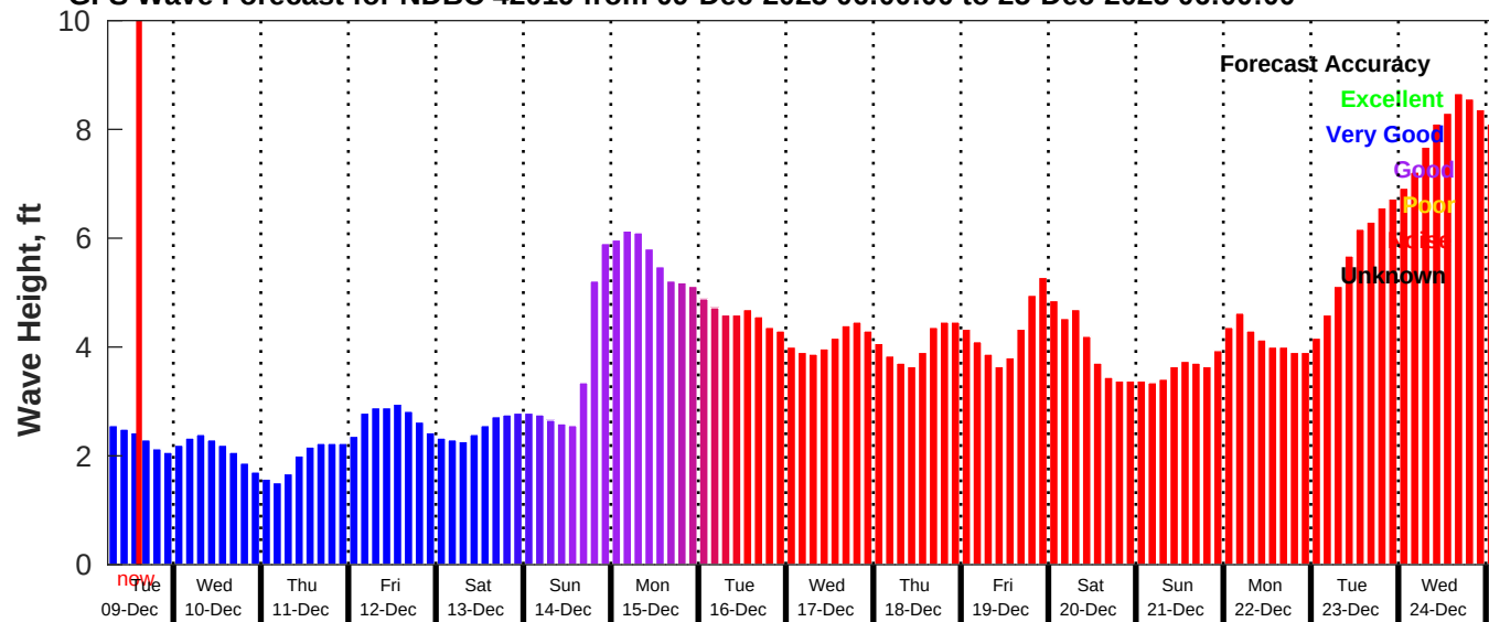
GFS Wave Forecast for NDBC 42019 from 09-Dec-2025 06:00:00 to 25-Dec-2025 06:00:00
