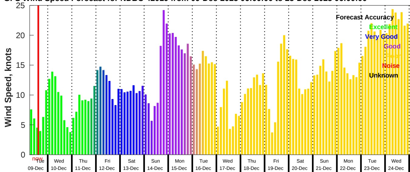
GFS Wind Speed Forecast for NDBC 42019 from 09-Dec-2025 06:00:00 to 25-Dec-2025 06:00:00
