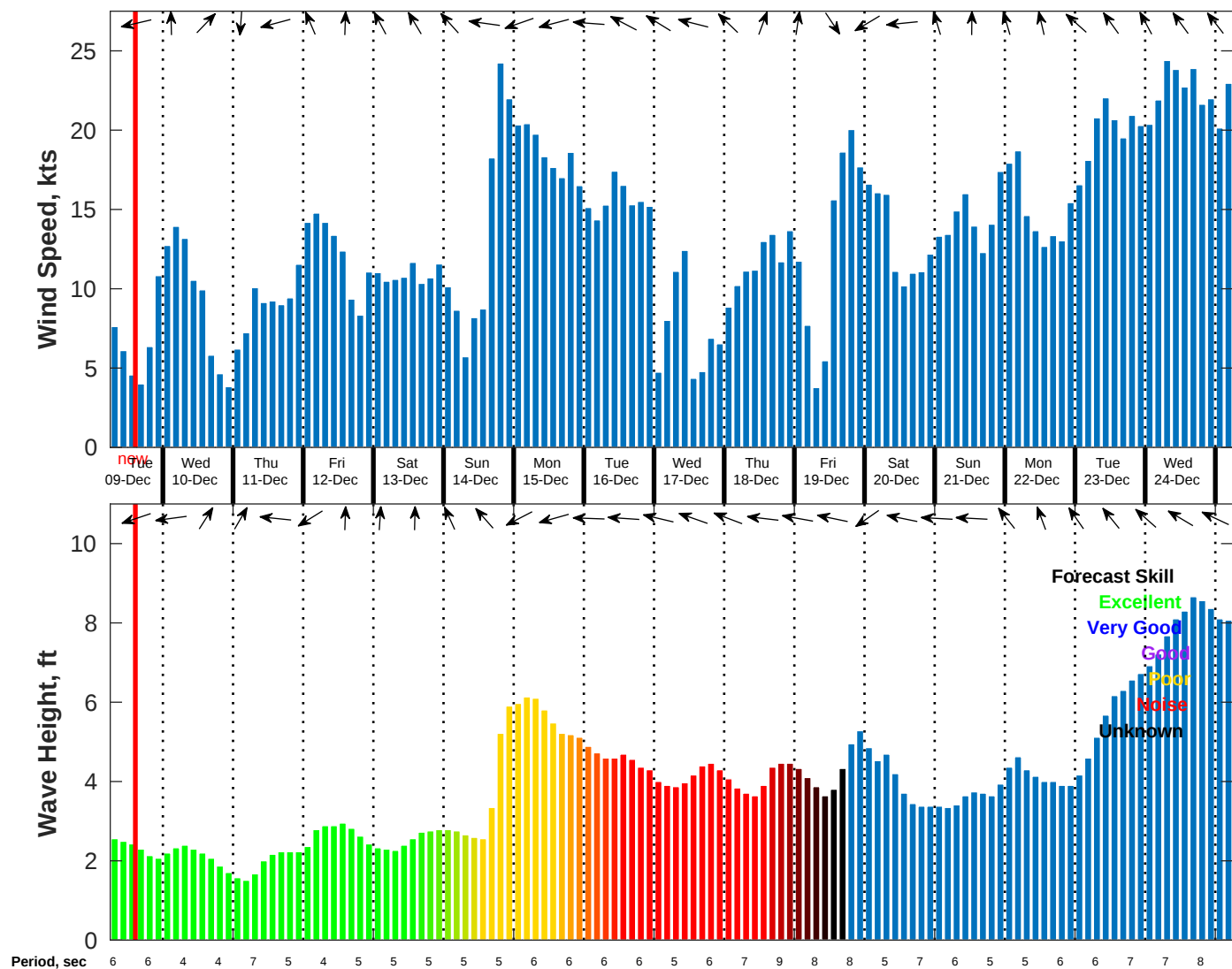
Wind & Wave Forecast for NDBC 42019 from 09-Dec-2025 06:00:00 to 25-Dec-2025 06:00:00
