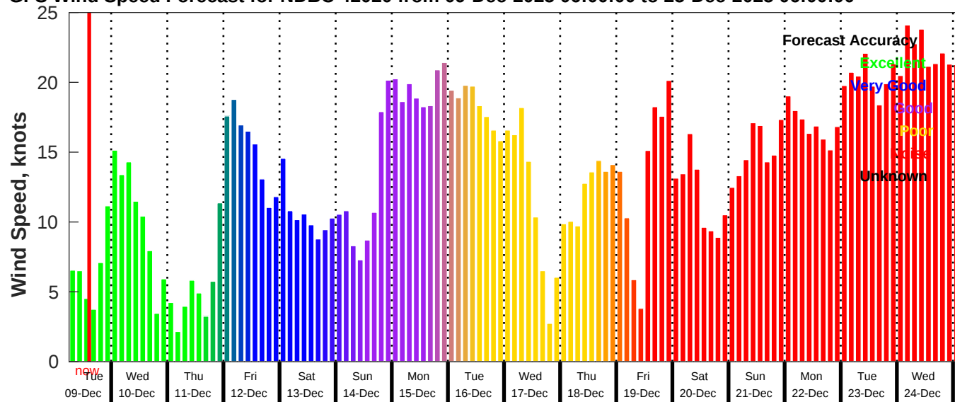
GFS Wind Speed Forecast for NDBC 42020 from 09-Dec-2025 06:00:00 to 25-Dec-2025 06:00:00
