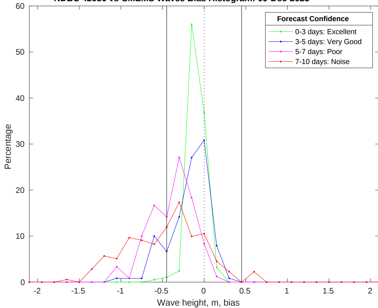
NDBC 42036 vs CMEMS Waves Bias Histogram: 09-Dec-2025
