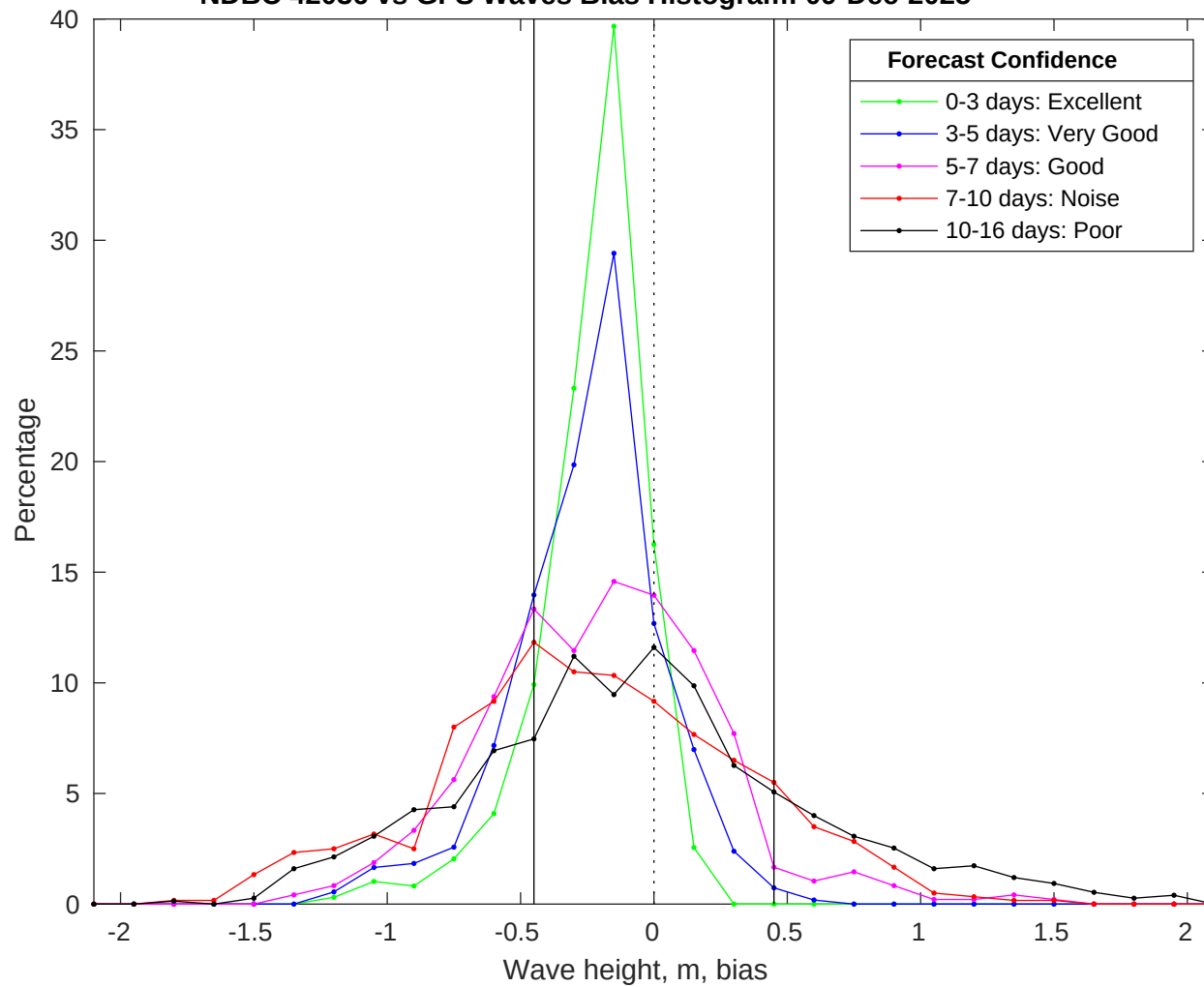
NDBC 42036 vs GFS Waves Bias Histogram: 09-Dec-2025
