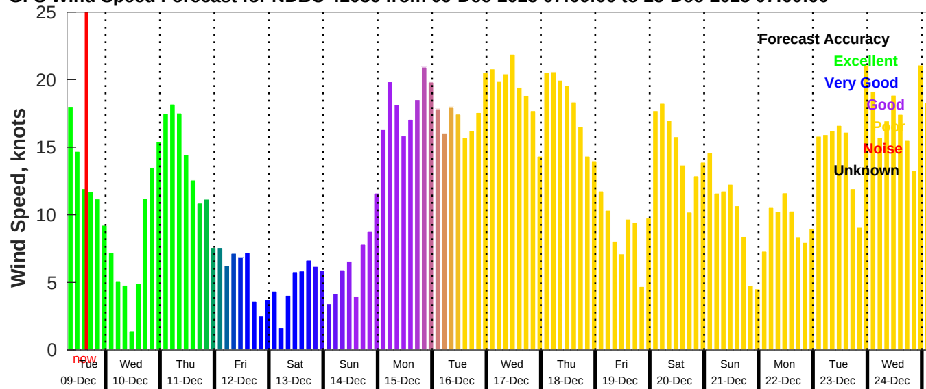
GFS Wind Speed Forecast for NDBC 42036 from 09-Dec-2025 07:00:00 to 25-Dec-2025 07:00:00
