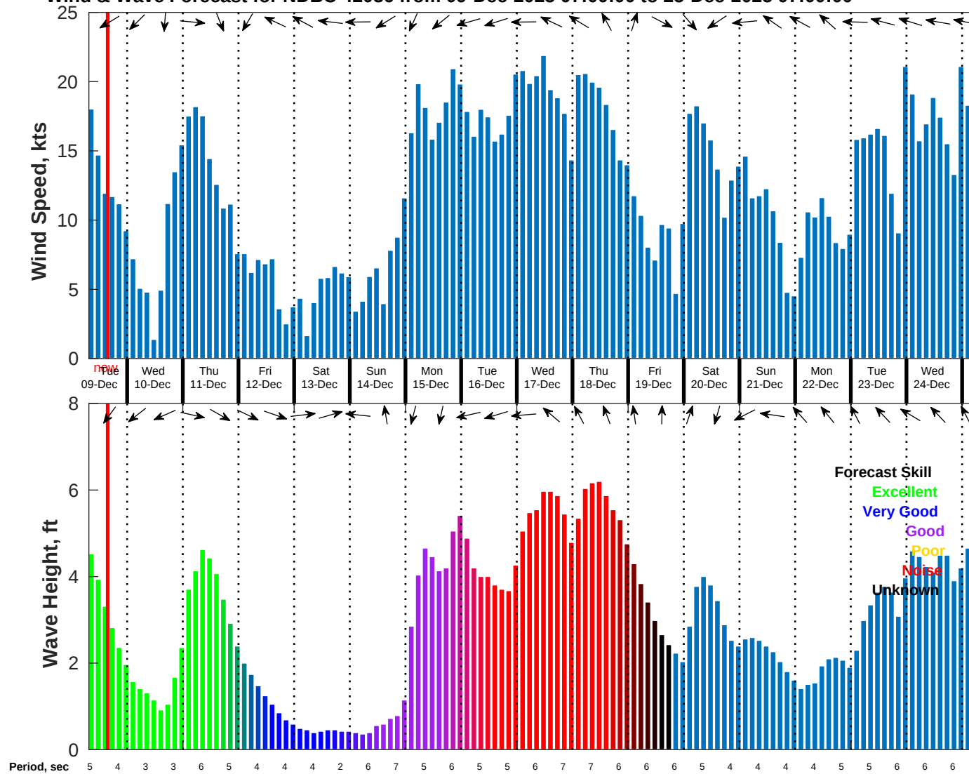
Wind & Wave Forecast for NDBC 42036 from 09-Dec-2025 07:00:00 to 25-Dec-2025 07:00:00
