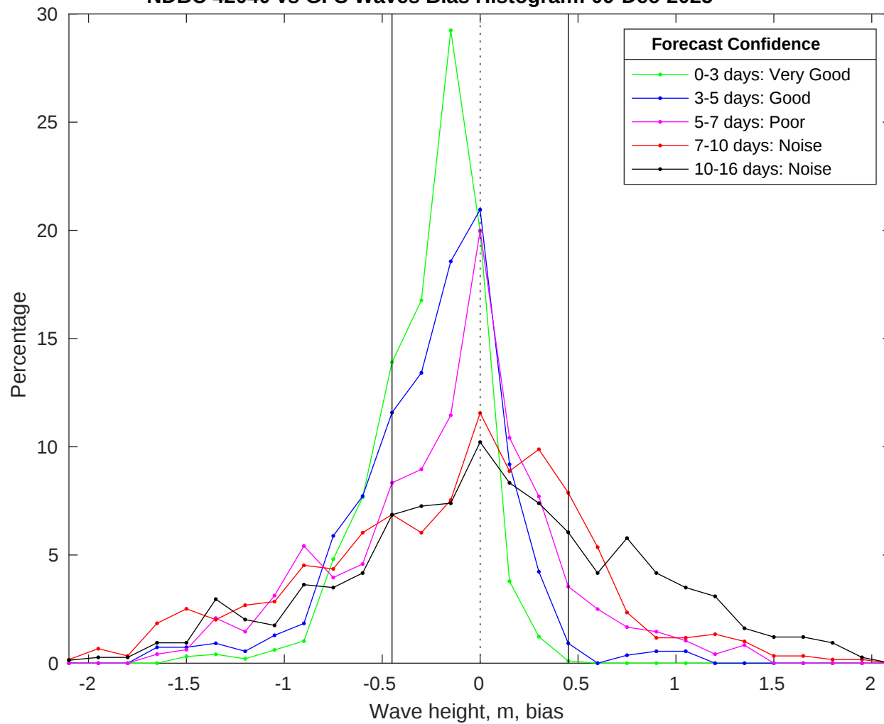
NDBC 42040 vs GFS Waves Bias Histogram: 09-Dec-2025
