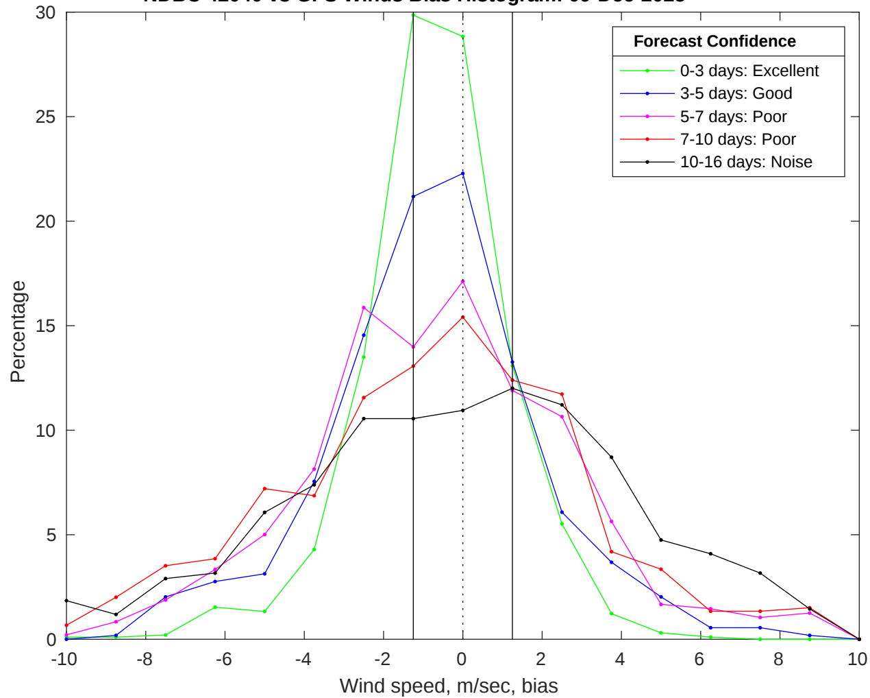
NDBC 42040 vs GFS Winds Bias Histogram: 09-Dec-2025
