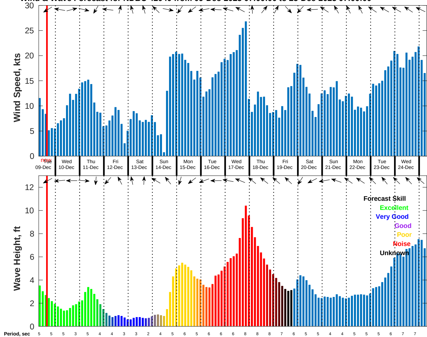
Wind & Wave Forecast for NDBC 42040 from 09-Dec-2025 07:00:00 to 25-Dec-2025 07:00:00
