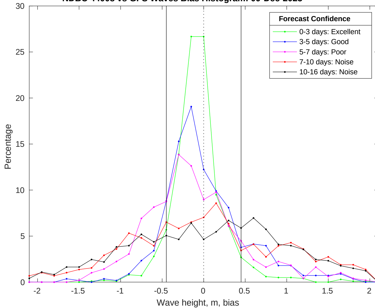
NDBC 44008 vs GFS Waves Bias Histogram: 09-Dec-2025
