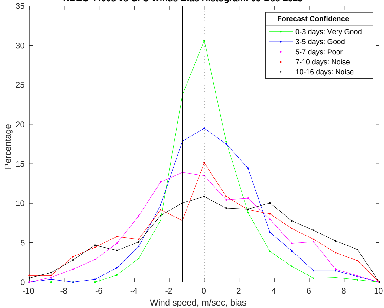
NDBC 44008 vs GFS Winds Bias Histogram: 09-Dec-2025
