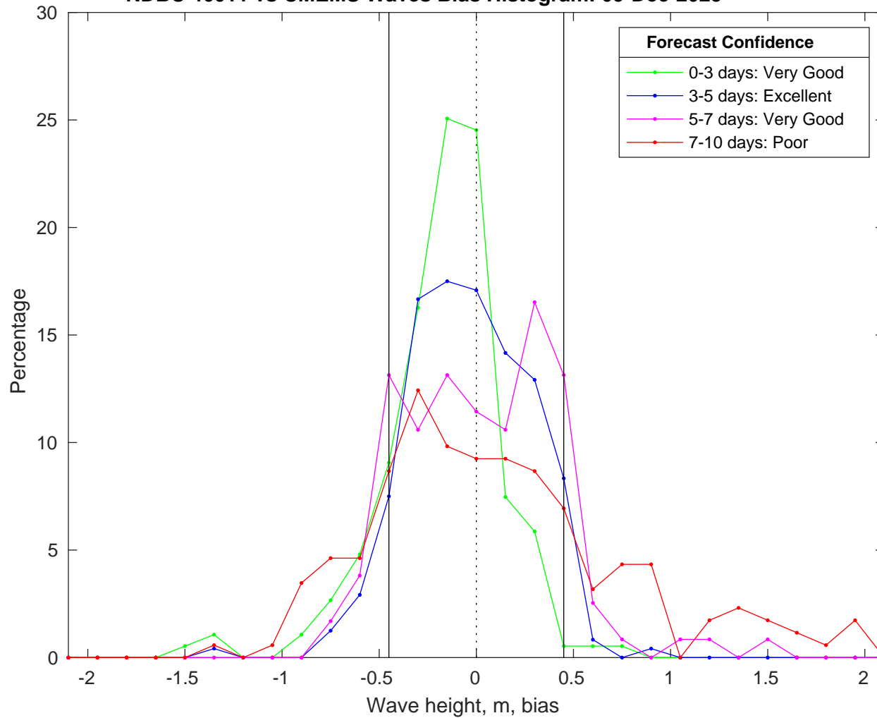
NDBC 46011 vs CMEMS Waves Bias Histogram: 09-Dec-2025
