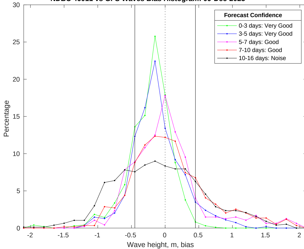
NDBC 46011 vs GFS Waves Bias Histogram: 09-Dec-2025
