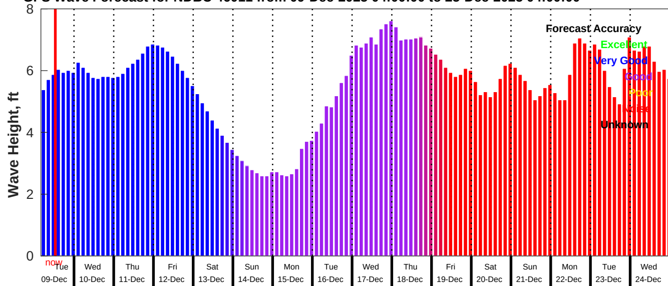
GFS Wave Forecast for NDBC 46011 from 09-Dec-2025 04:00:00 to 25-Dec-2025 04:00:00
