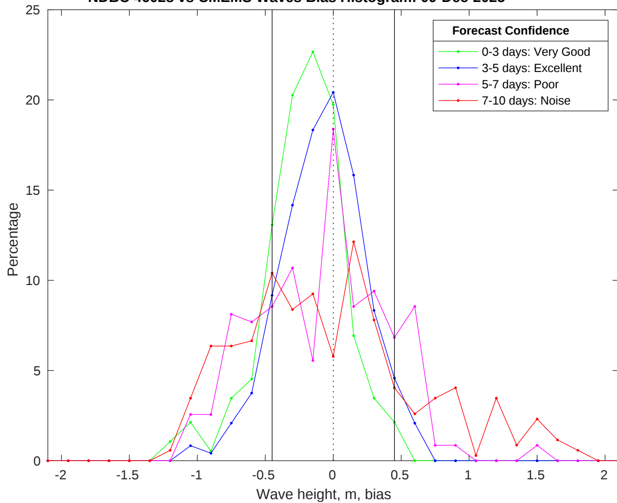
NDBC 46028 vs CMEMS Waves Bias Histogram: 09-Dec-2025
