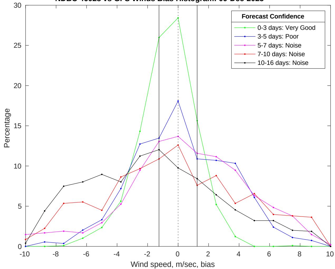
NDBC 46028 vs GFS Winds Bias Histogram: 09-Dec-2025
