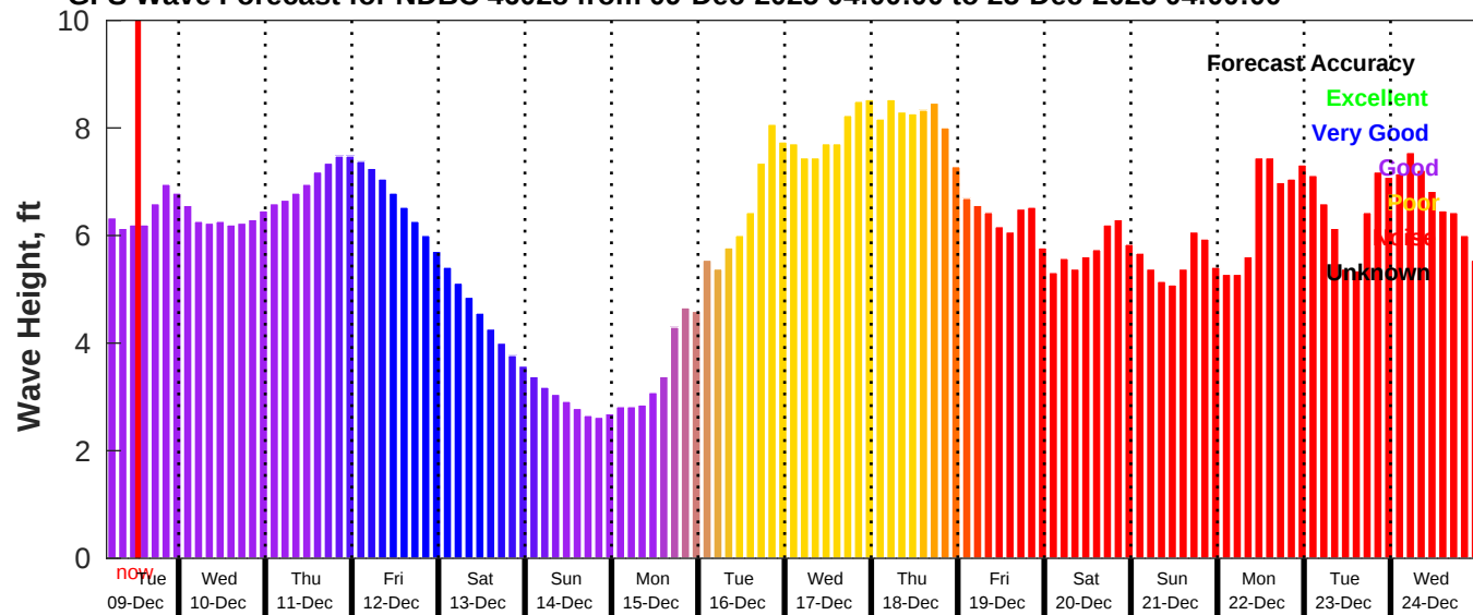
GFS Wave Forecast for NDBC 46028 from 09-Dec-2025 04:00:00 to 25-Dec-2025 04:00:00
