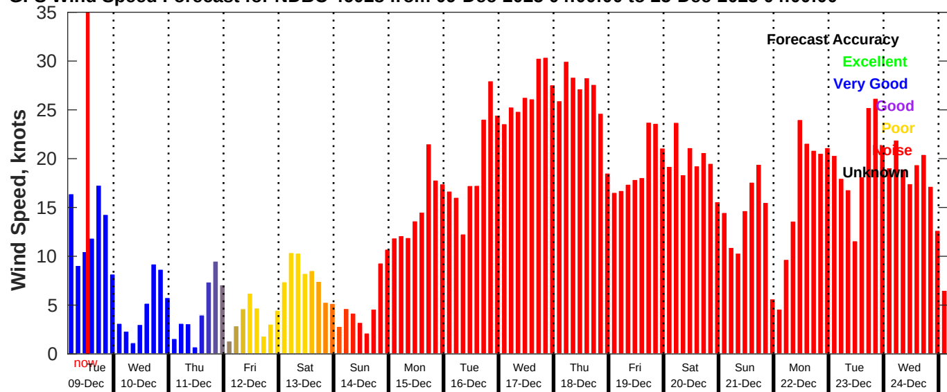
GFS Wind Speed Forecast for NDBC 46028 from 09-Dec-2025 04:00:00 to 25-Dec-2025 04:00:00
