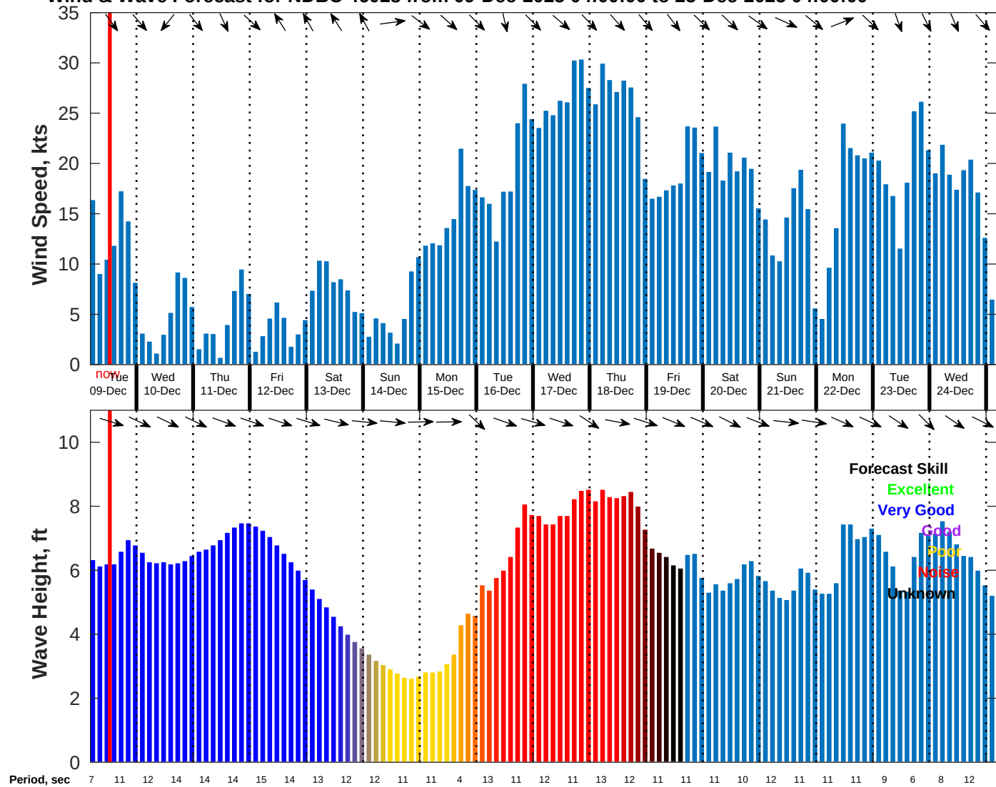
Wind & Wave Forecast for NDBC 46028 from 09-Dec-2025 04:00:00 to 25-Dec-2025 04:00:00
