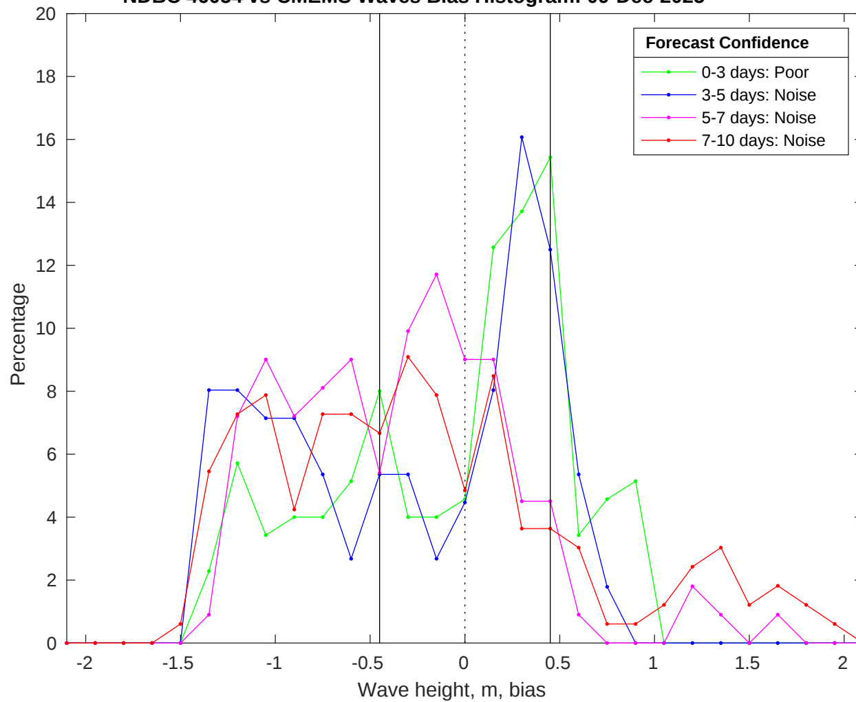
NDBC 46054 vs CMEMS Waves Bias Histogram: 09-Dec-2025
