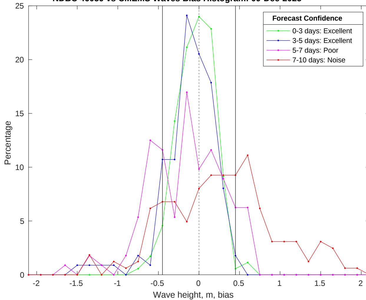
NDBC 46059 vs CMEMS Waves Bias Histogram: 09-Dec-2025
