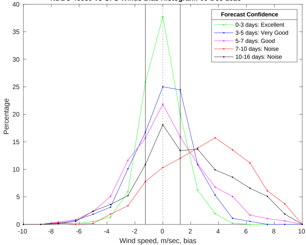
NDBC 46059 vs GFS Winds Bias Histogram: 09-Dec-2025
