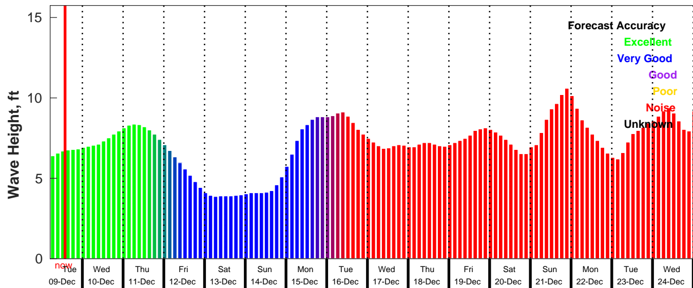
GFS Wave Forecast for NDBC 46059 from 09-Dec-2025 05:00:00 to 25-Dec-2025 05:00:00
