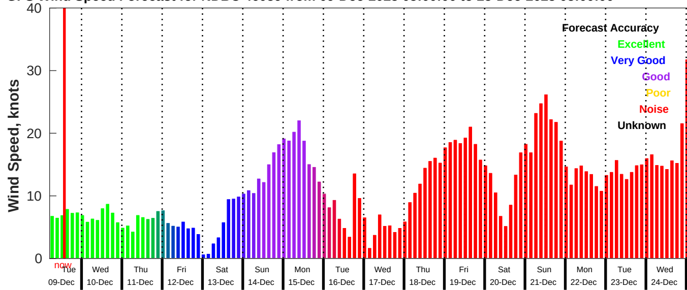
GFS Wind Speed Forecast for NDBC 46059 from 09-Dec-2025 05:00:00 to 25-Dec-2025 05:00:00
