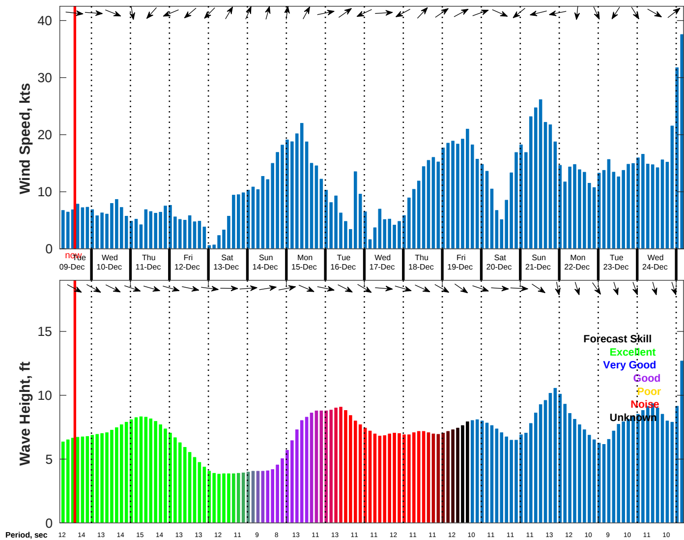
Wind & Wave Forecast for NDBC 46059 from 09-Dec-2025 05:00:00 to 25-Dec-2025 05:00:00
