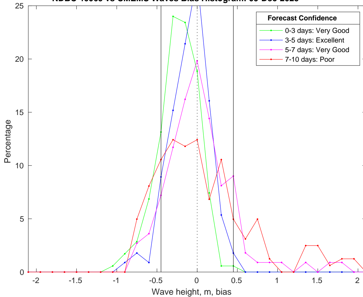
NDBC 46069 vs CMEMS Waves Bias Histogram: 09-Dec-2025
