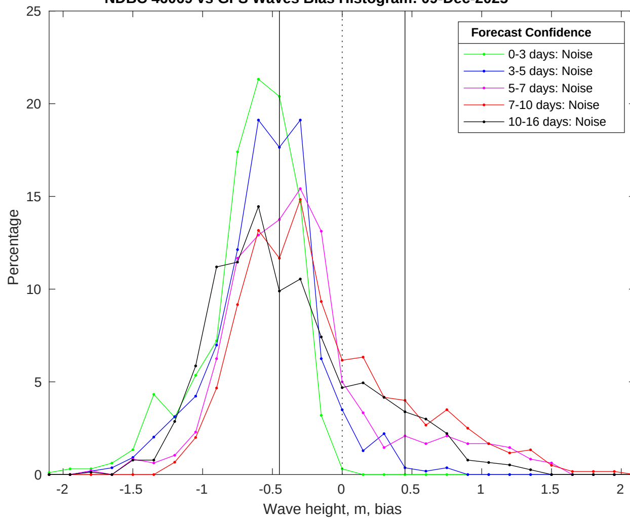
NDBC 46069 vs GFS Waves Bias Histogram: 09-Dec-2025
