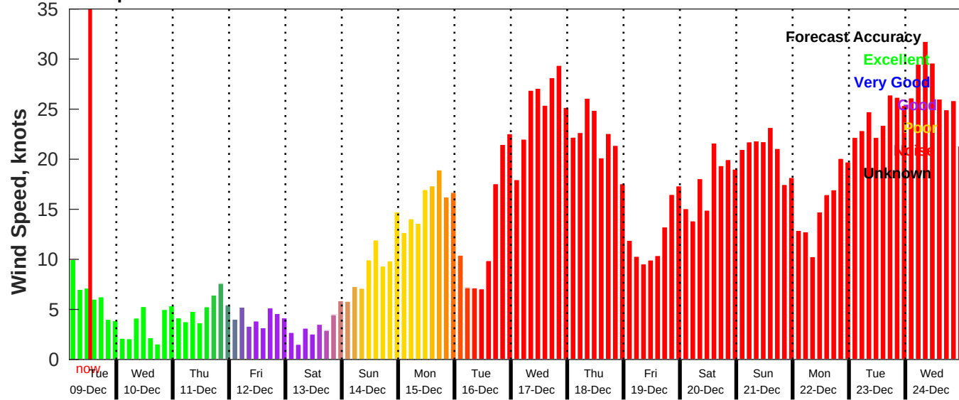
GFS Wind Speed Forecast for NDBC 46069 from 09-Dec-2025 04:00:00 to 25-Dec-2025 04:00:00
