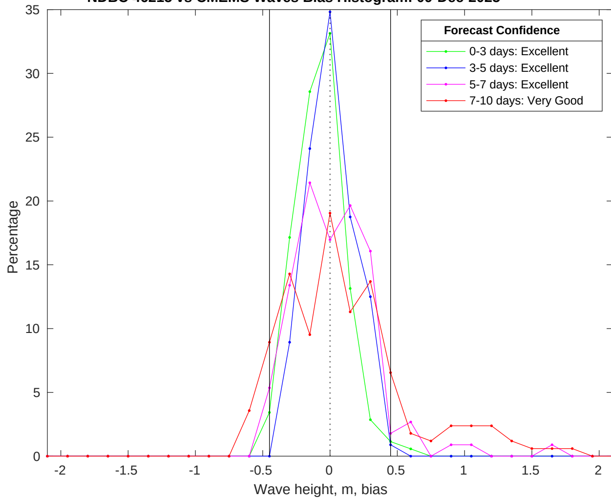
NDBC 46215 vs CMEMS Waves Bias Histogram: 09-Dec-2025
