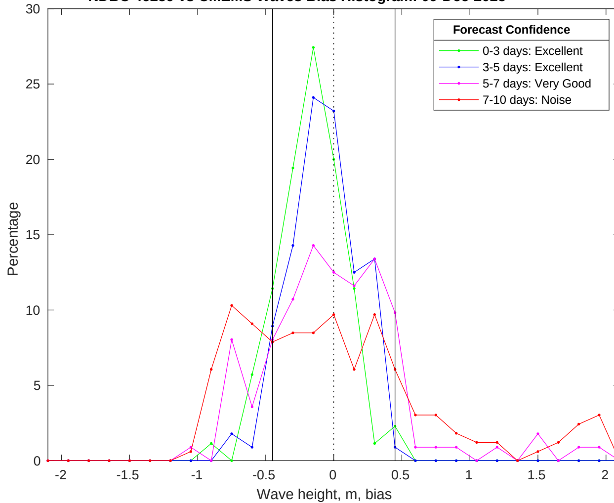
NDBC 46259 vs CMEMS Waves Bias Histogram: 09-Dec-2025
