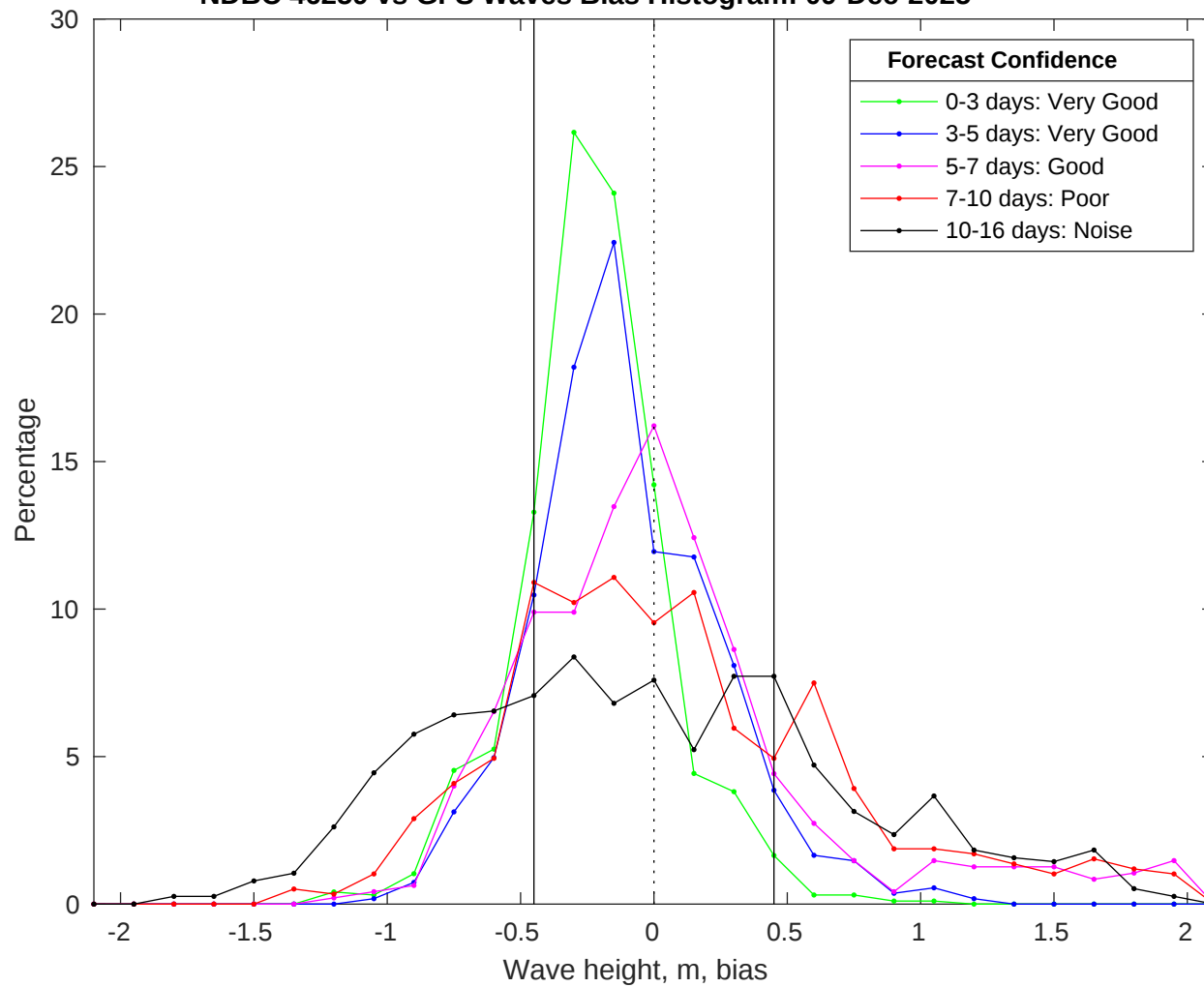
NDBC 46259 vs GFS Waves Bias Histogram: 09-Dec-2025
