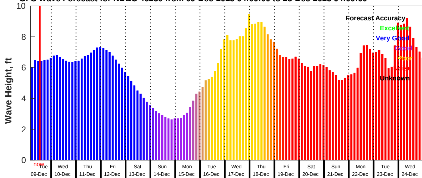
GFS Wave Forecast for NDBC 46259 from 09-Dec-2025 04:00:00 to 25-Dec-2025 04:00:00
