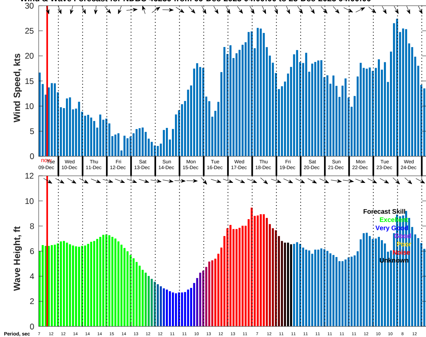
Wind & Wave Forecast for NDBC 46259 from 09-Dec-2025 04:00:00 to 25-Dec-2025 04:00:00
