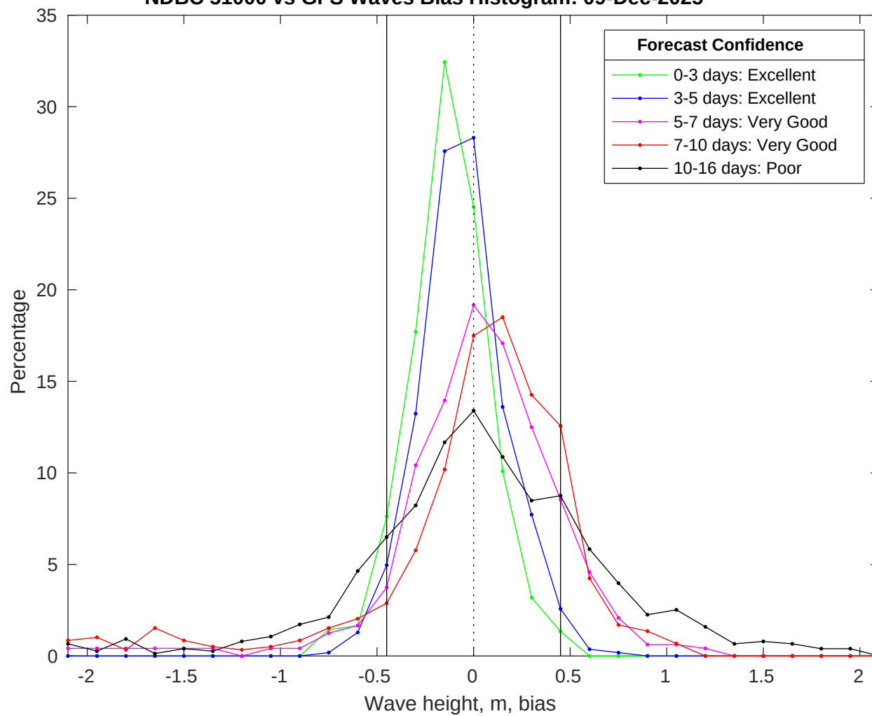
NDBC 51000 vs GFS Waves Bias Histogram: 09-Dec-2025
