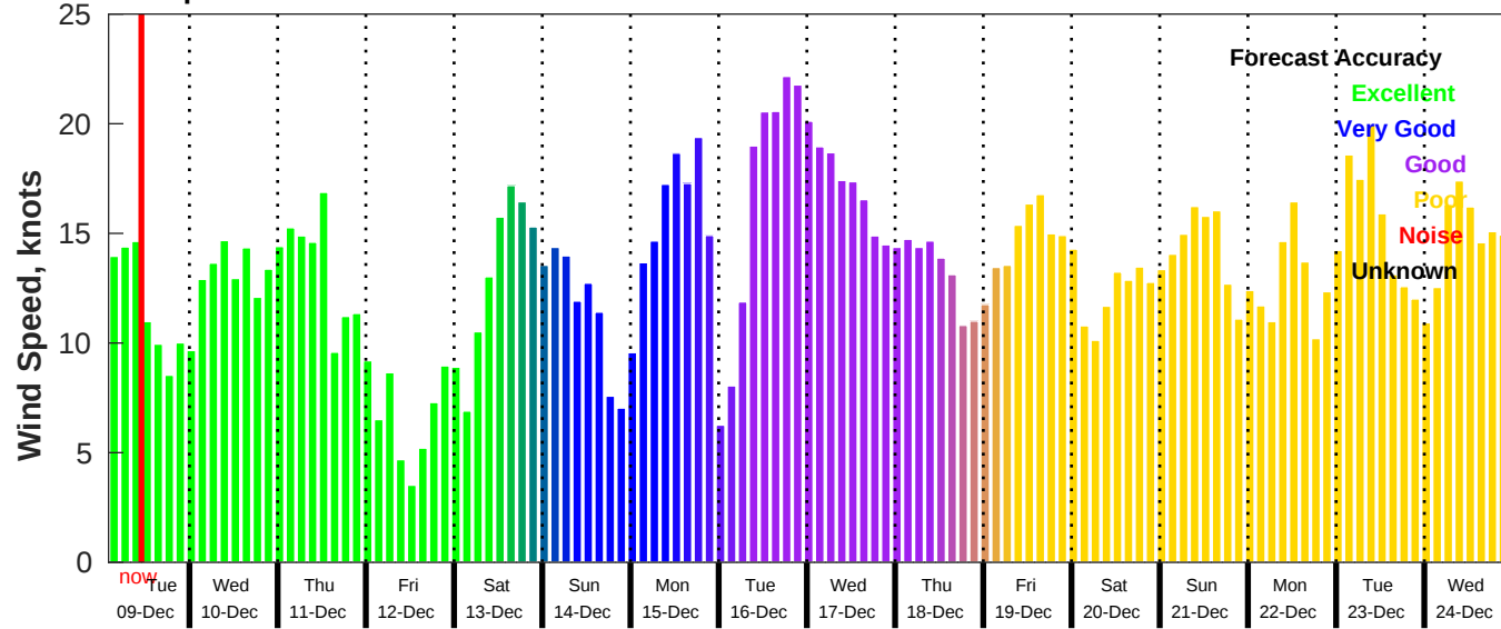
GFS Wind Speed Forecast for NDBC 51000 from 09-Dec-2025 02:00:00 to 25-Dec-2025 02:00:00
