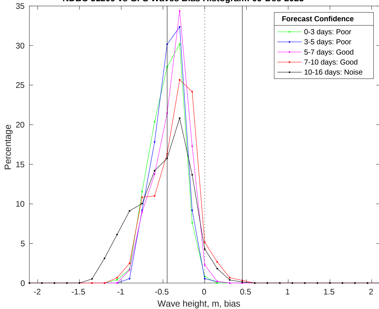
NDBC 51209 vs GFS Waves Bias Histogram: 09-Dec-2025
