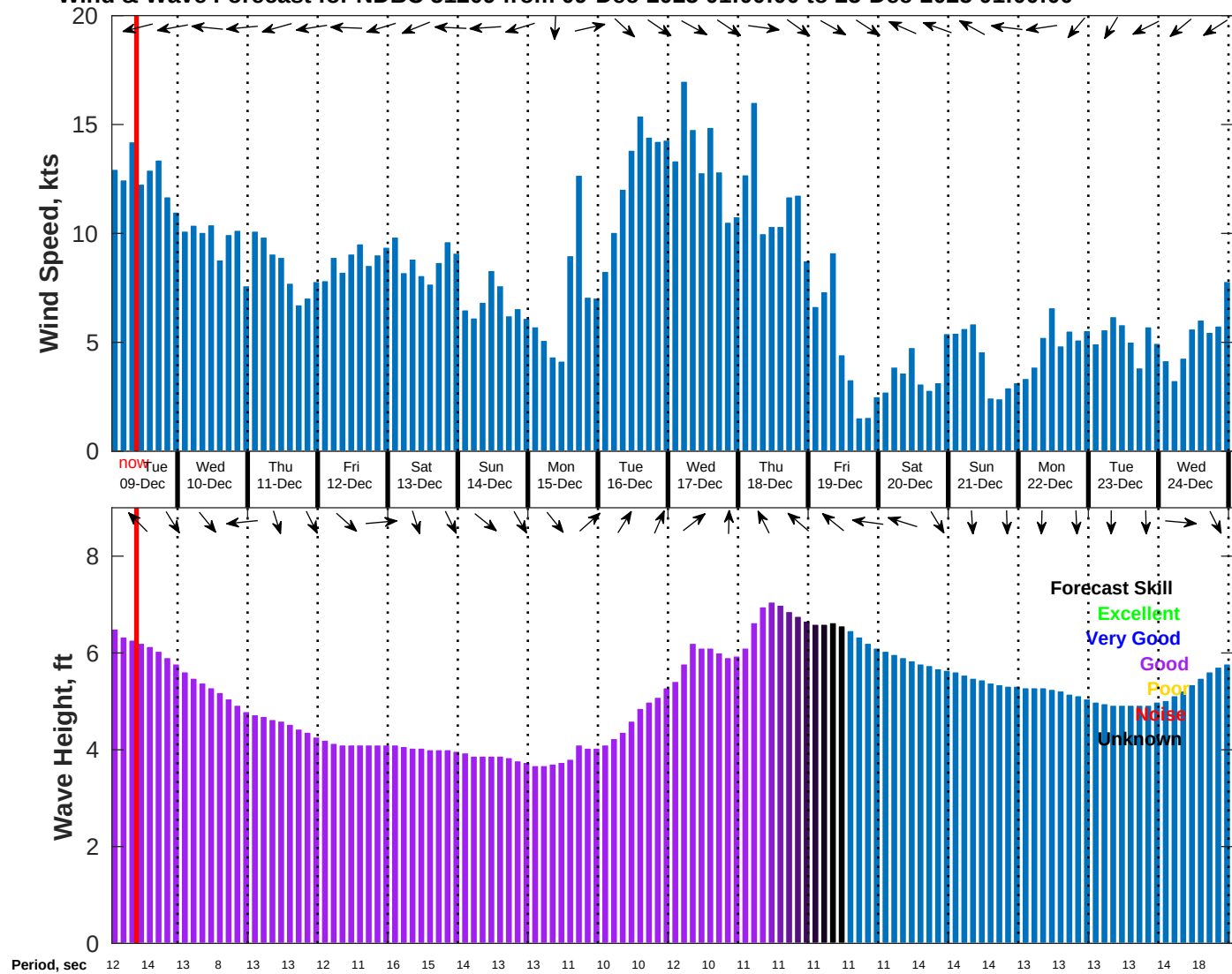
Wind & Wave Forecast for NDBC 51209 from 09-Dec-2025 01:00:00 to 25-Dec-2025 01:00:00
