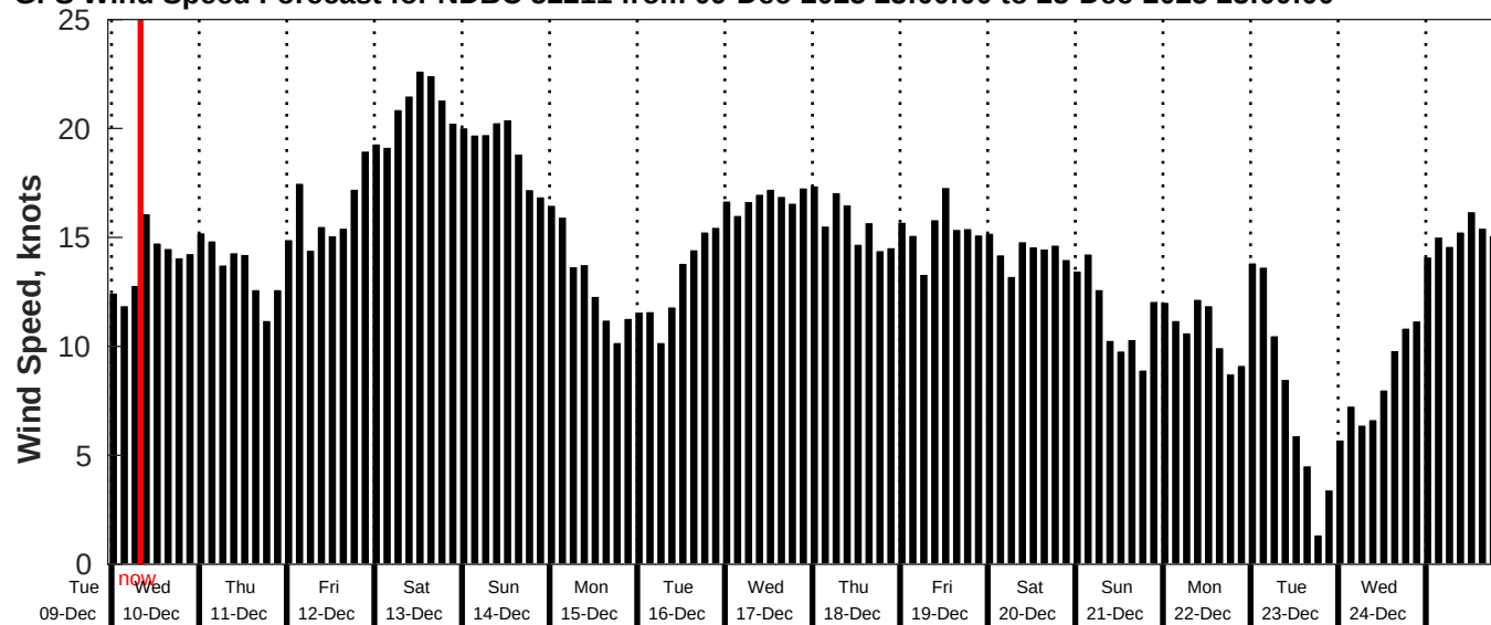
GFS Wind Speed Forecast for NDBC 52211 from 09-Dec-2025 23:00:00 to 25-Dec-2025 23:00:00
