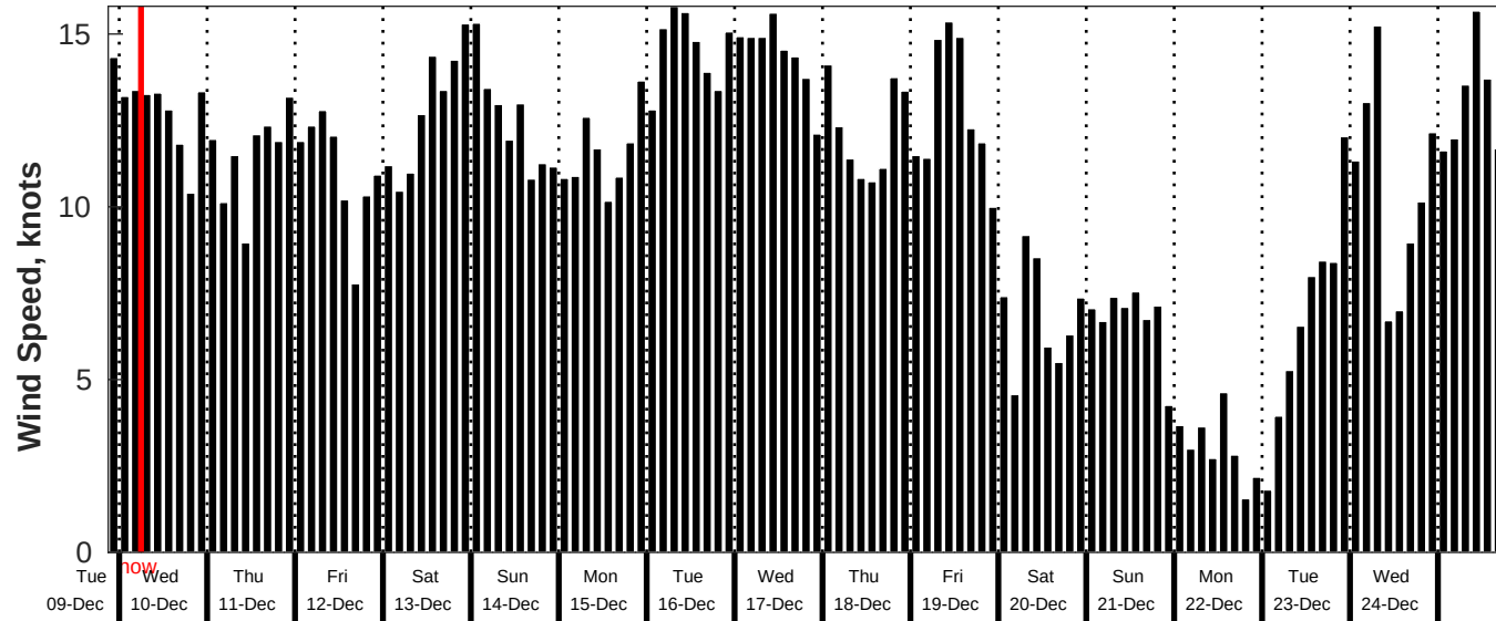
GFS Wind Speed Forecast for NDBC 52212 from 09-Dec-2025 21:00:00 to 25-Dec-2025 21:00:00
