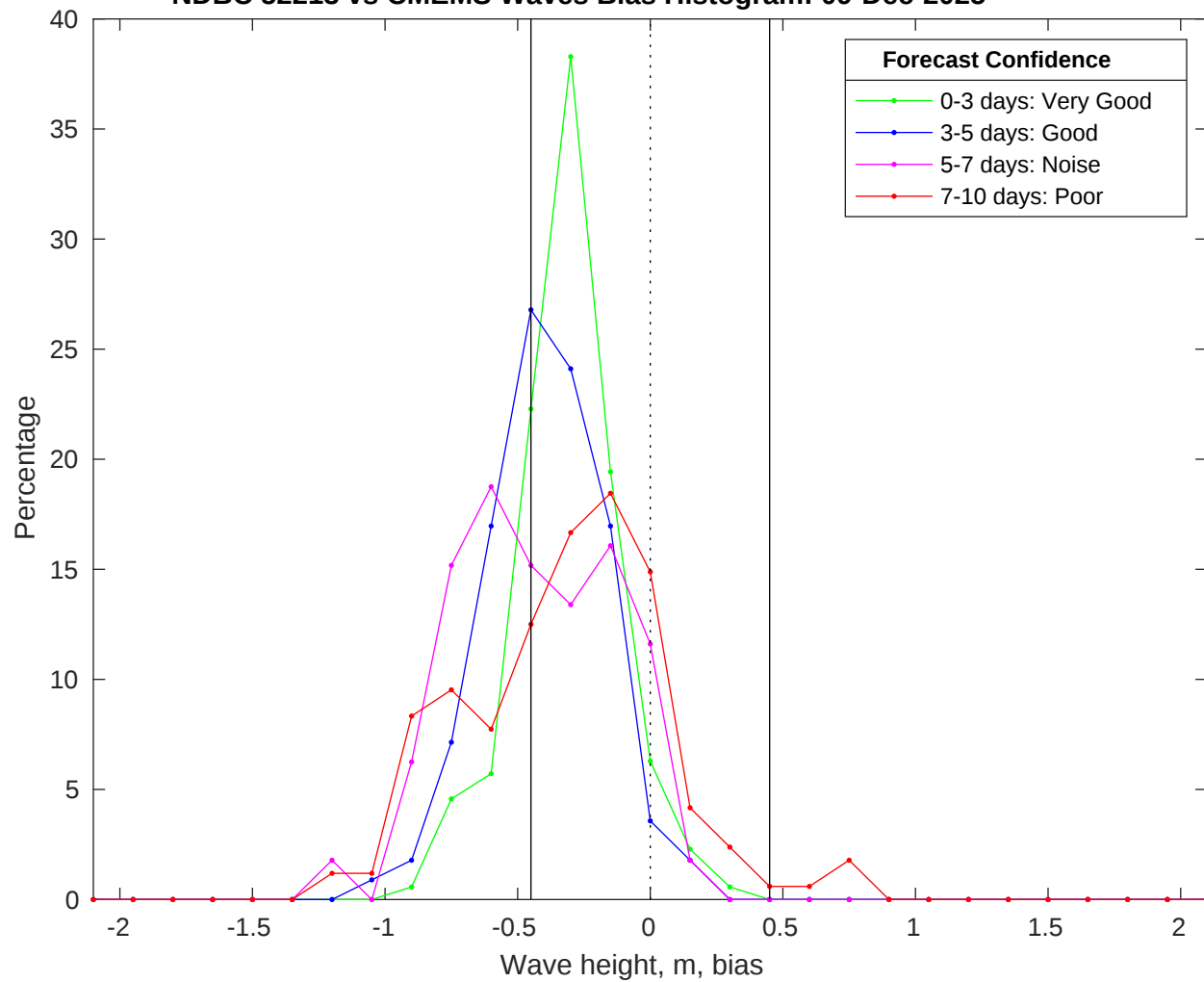
NDBC 52213 vs CMEMS Waves Bias Histogram: 09-Dec-2025
