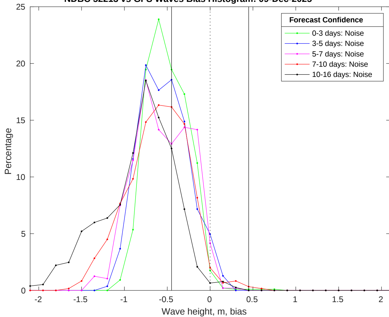
NDBC 52213 vs GFS Waves Bias Histogram: 09-Dec-2025
