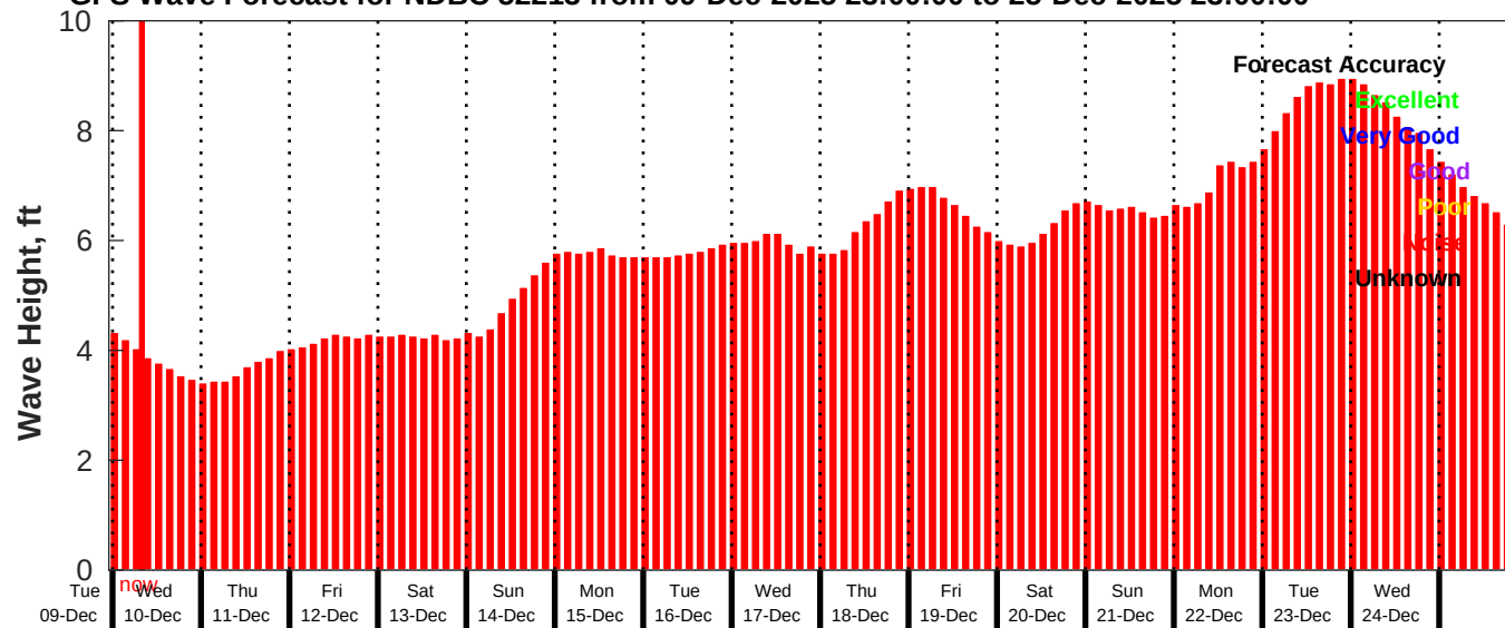
GFS Wave Forecast for NDBC 52213 from 09-Dec-2025 23:00:00 to 25-Dec-2025 23:00:00
