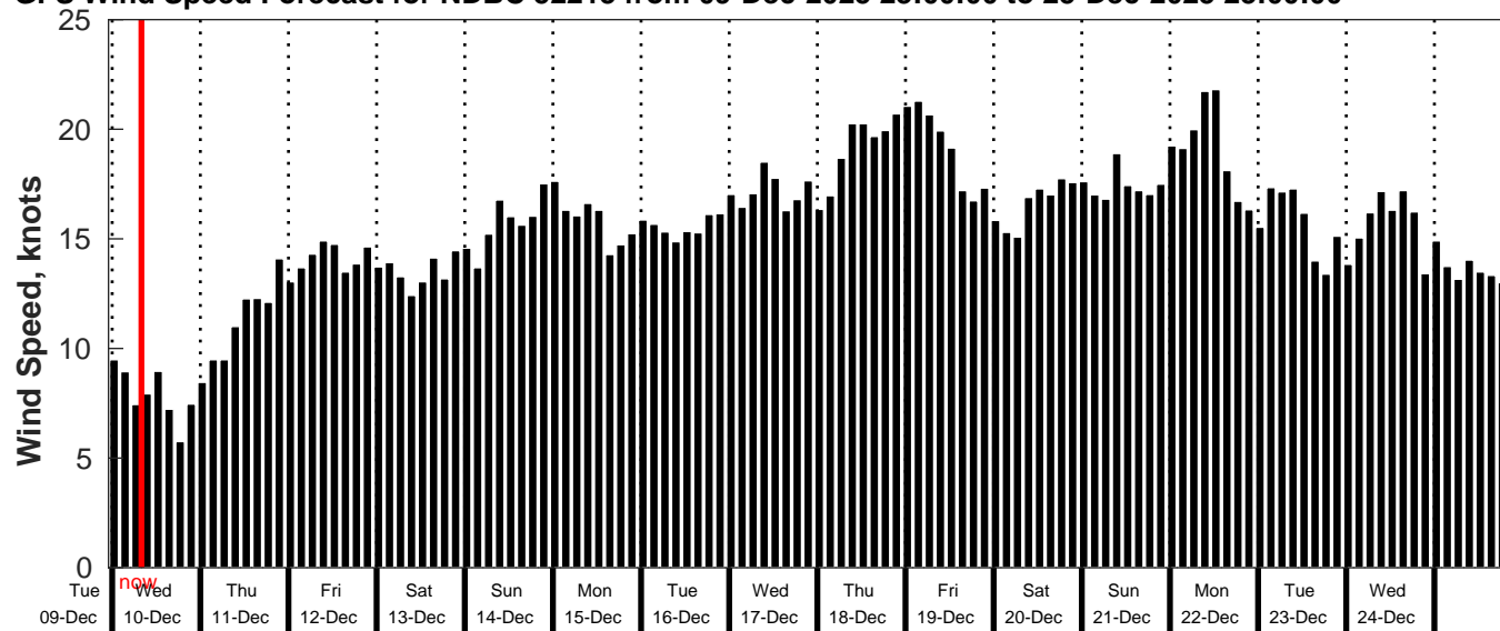
GFS Wind Speed Forecast for NDBC 52213 from 09-Dec-2025 23:00:00 to 25-Dec-2025 23:00:00
